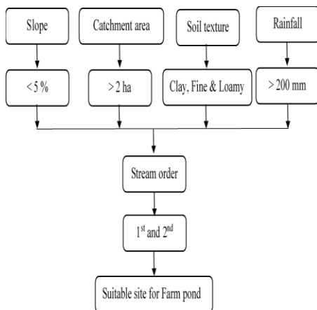
Fig. 12. Site selection criteria for farm pond
