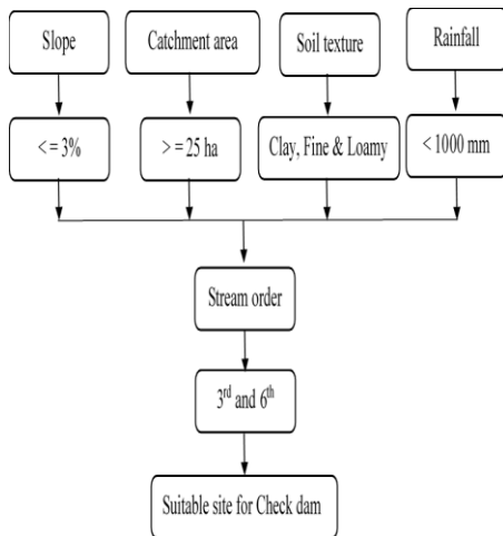
Fig. 10. Site selection criteria for check dam
