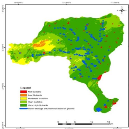
Fig. 13. Model suitability validation map of RWH site
