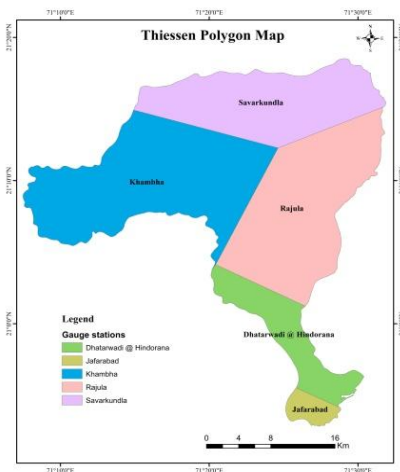
Fig. 2. Thiessen polygon map of rainfall for
