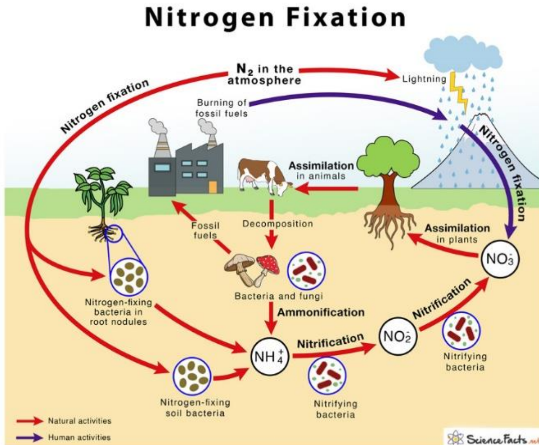
Fig. 1. Nitrogen fixation
