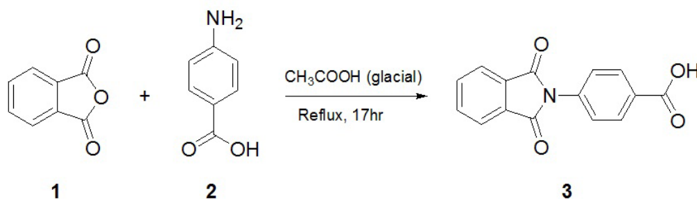
Figure 2. Reagents and conditions for the synthesis of N-(4-carboxyphenyl)phthalimide (3).
