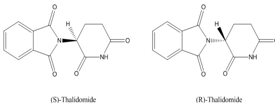
Figure 1. Thalidomide enantiomers.
