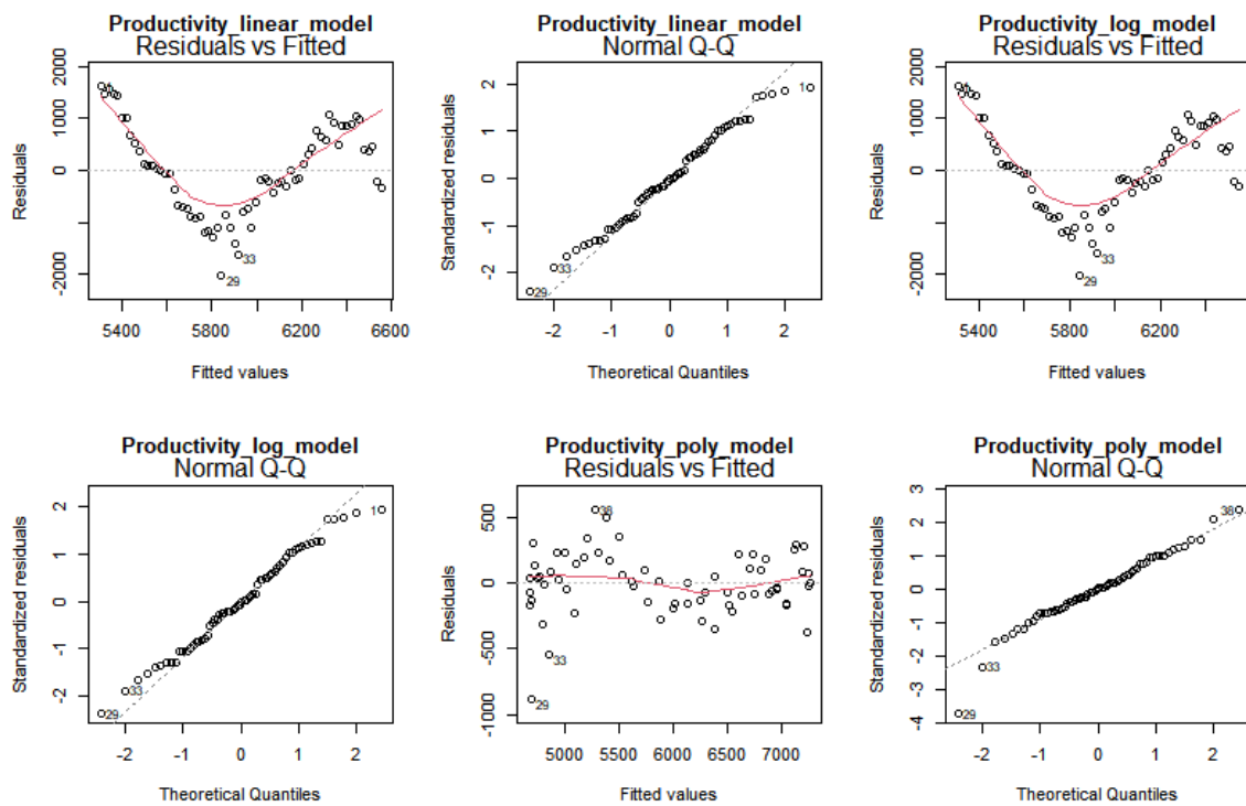
Fig. 5. residual vs. fitted and Q-Q plots of various regression models for production of coconut in Kerala
