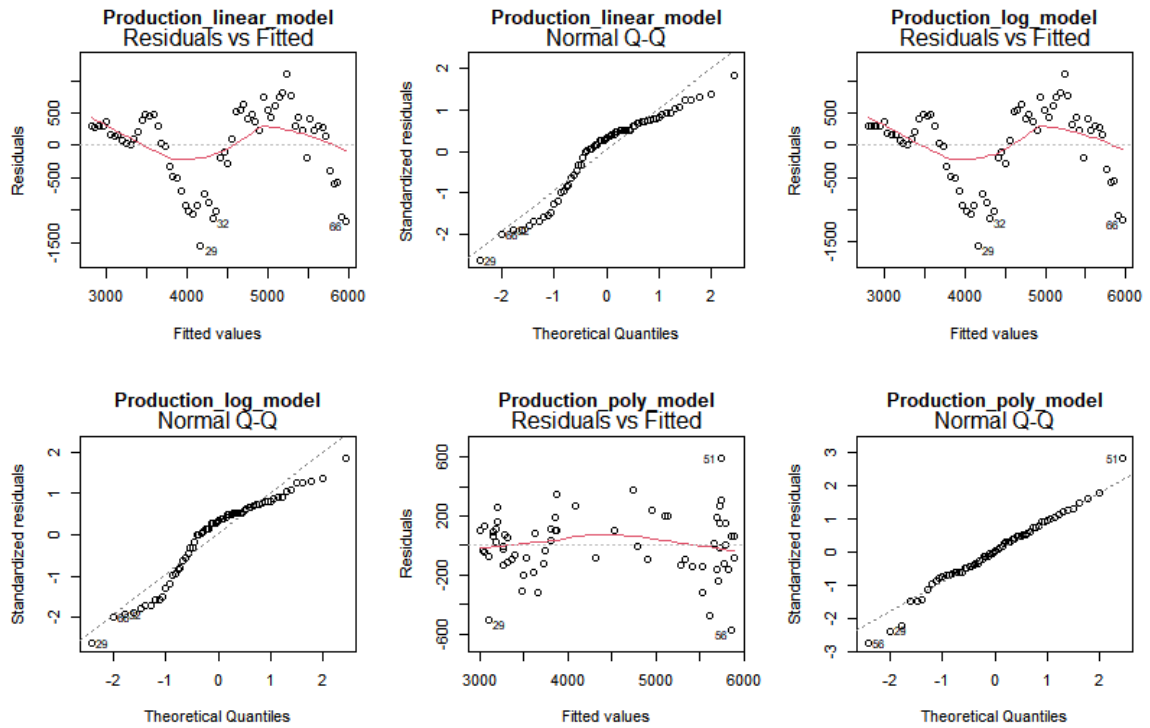
Fig. 4. residual vs. fitted and Q-Q plots of various regression models for production of coconut in Kerala
