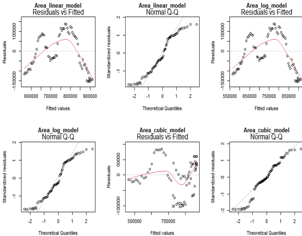
Fig..3. residual vs. fitted and Q-Q plots of various regression models for Area of coconut production in Kerala
