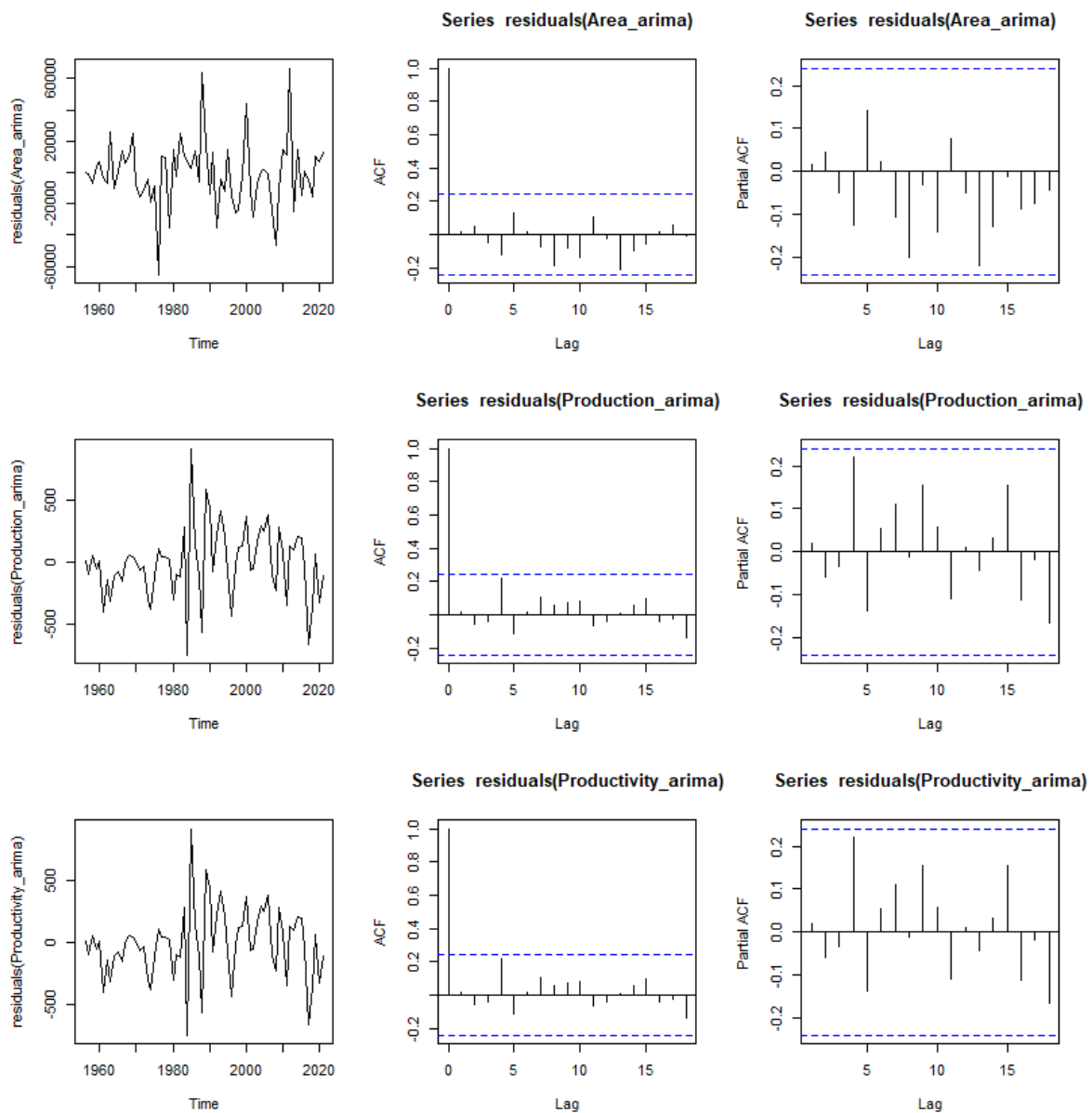
Fig..2. The residual plots, acf plots, and pacf plots for ARIMA models
