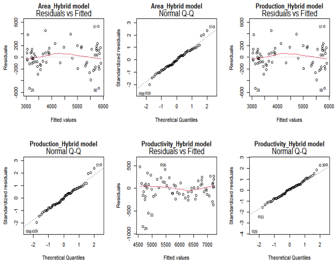
Fig. 6. residual vs. fitted and Q-Q plots of Hybrid model for Area of coconut production in Kerala
