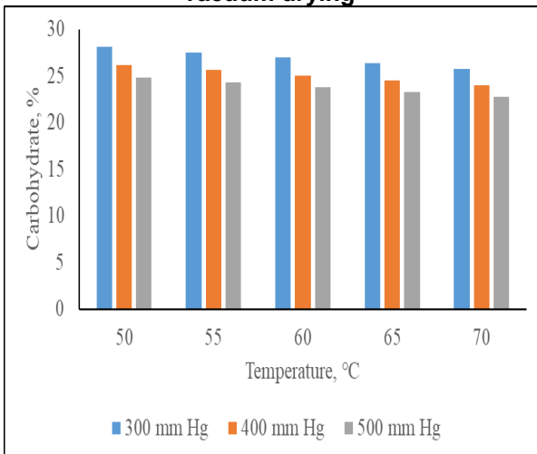
Fig. 1(e). Effect on carbohydrate content during vacuum drying
