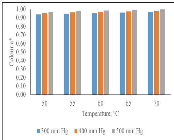
Fig. 1(g). Effect on colour a* value using vacuum drying
