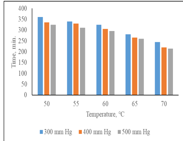
Fig. 1(b). Effect on drying time during vacuum drying
