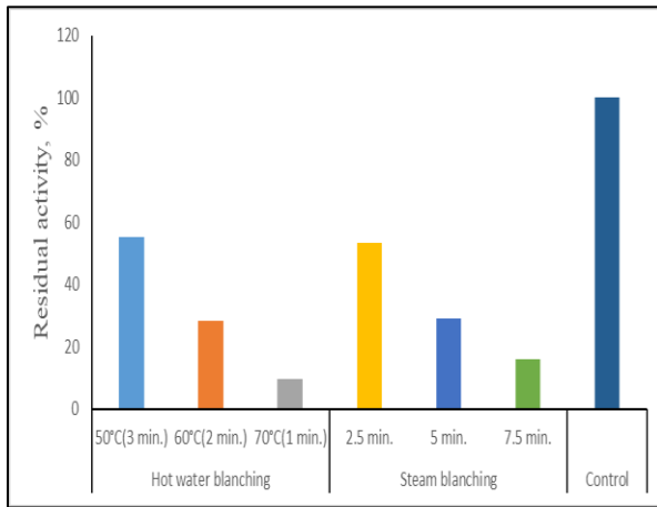
Fig. 1(a). Effect on Residual activity during blanching
