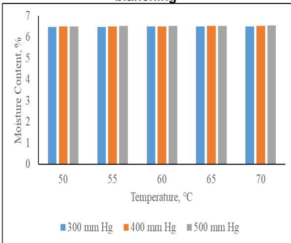
Fig. 1(c). Effect on moisture content during vacuum drying
