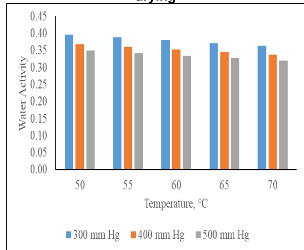
Fig. 1(d). Effect on water activity during vacuum drying
