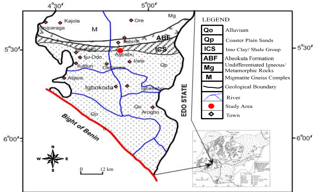
Fig. 1. Geological map of southern part of Ondo state showing the study area (Modified After PTF, 1997)
