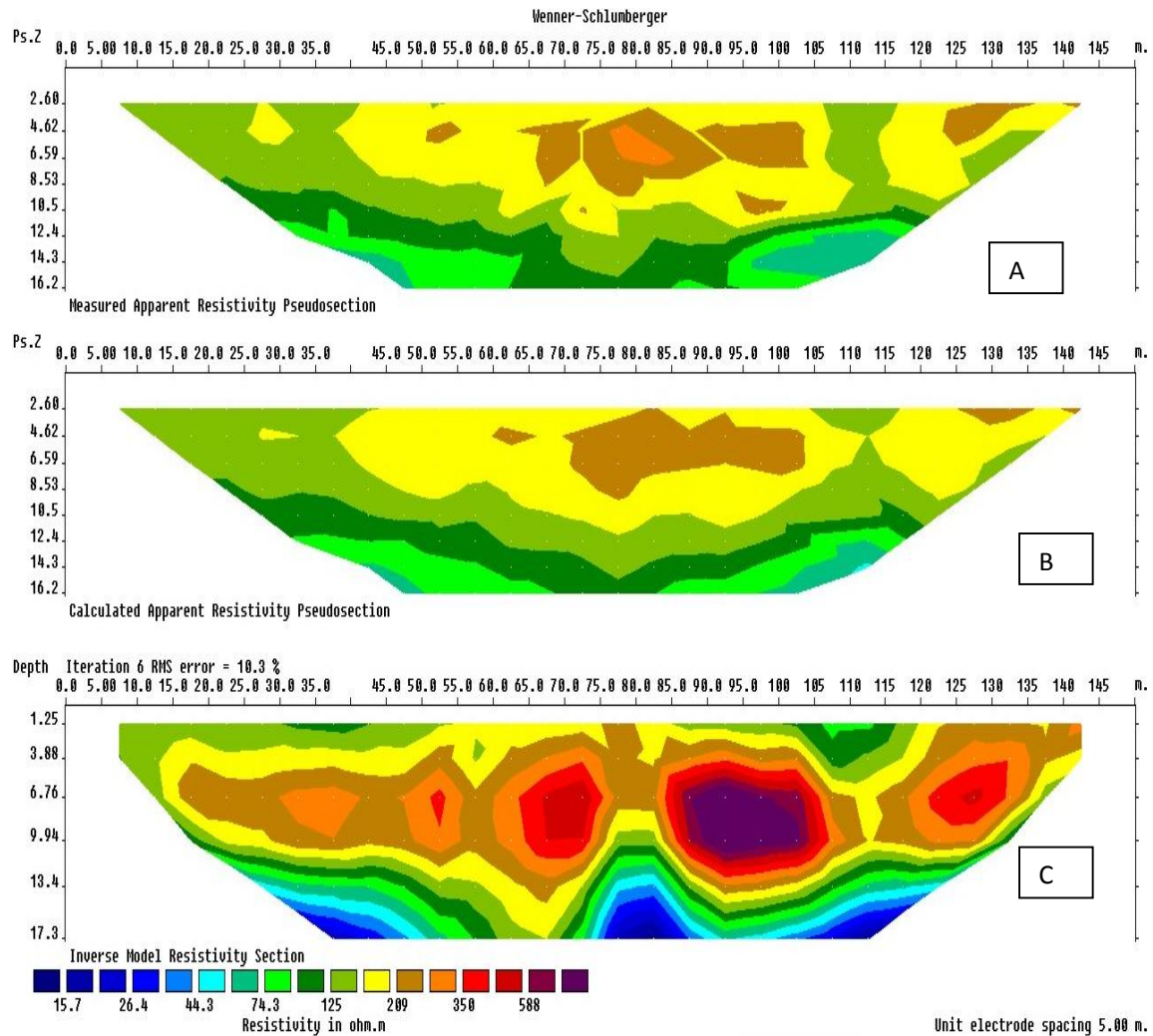
Fig. 3. Inverted 2D-resistivity section along traverse one
