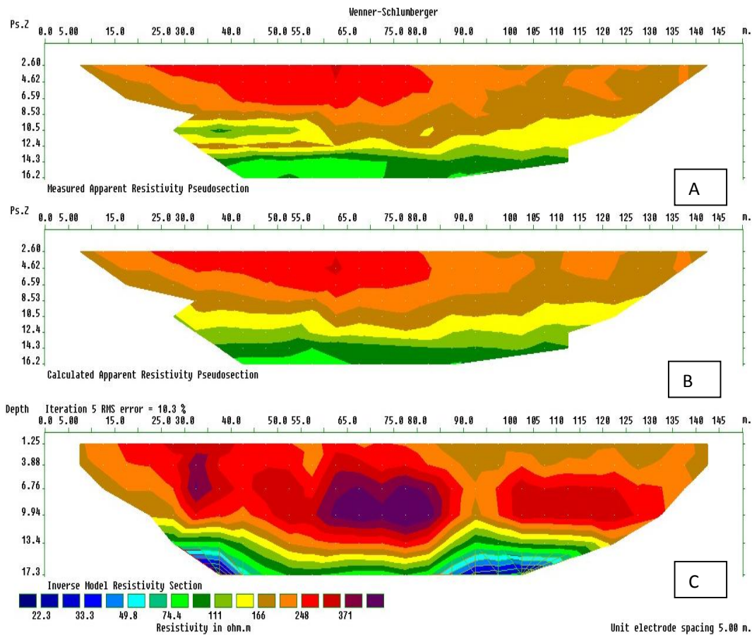
Fig. 4. Inverted 2D-resistivity section along traverse two
