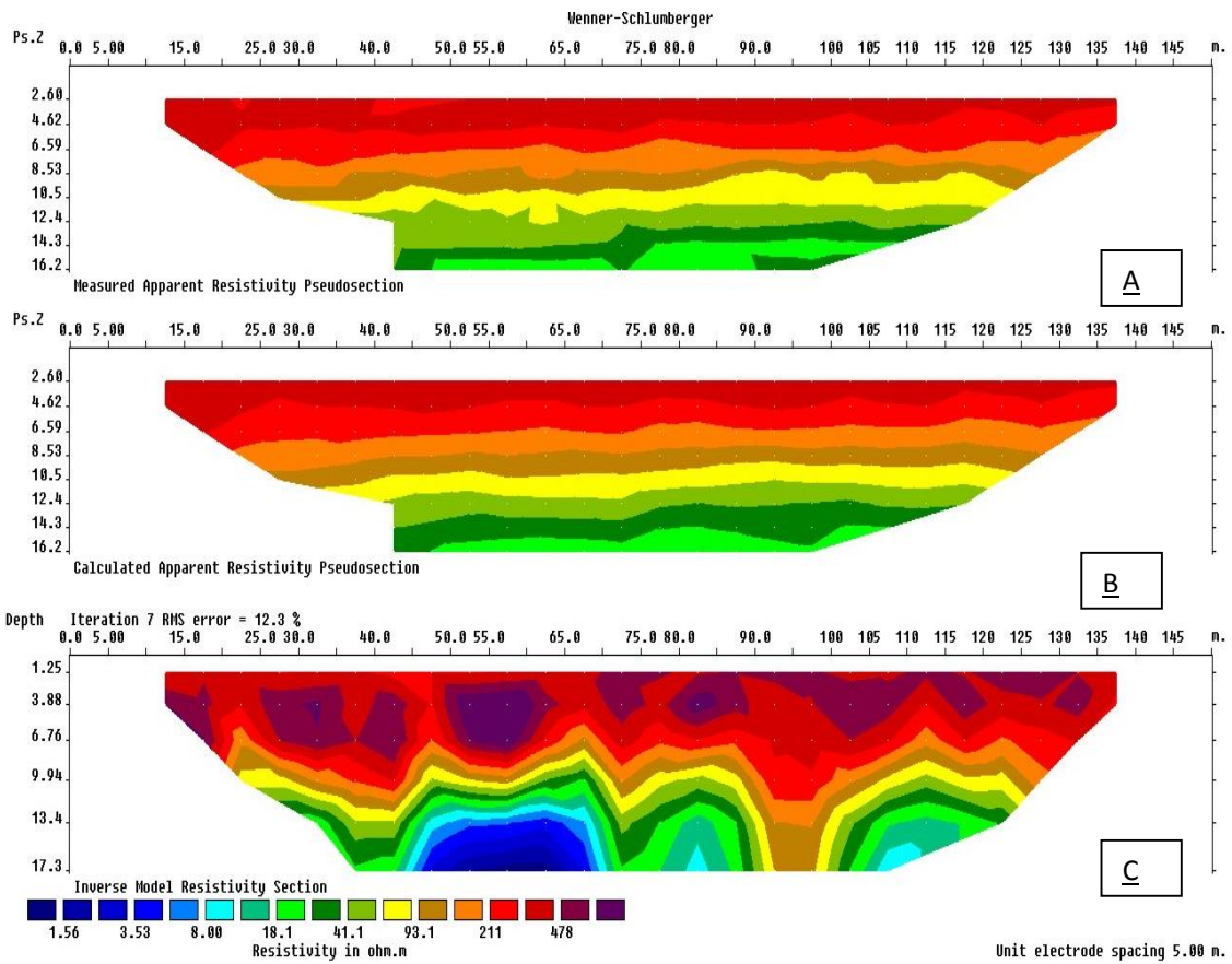
Fig. 8. Inverted 2D-resistivity section along traverse five
