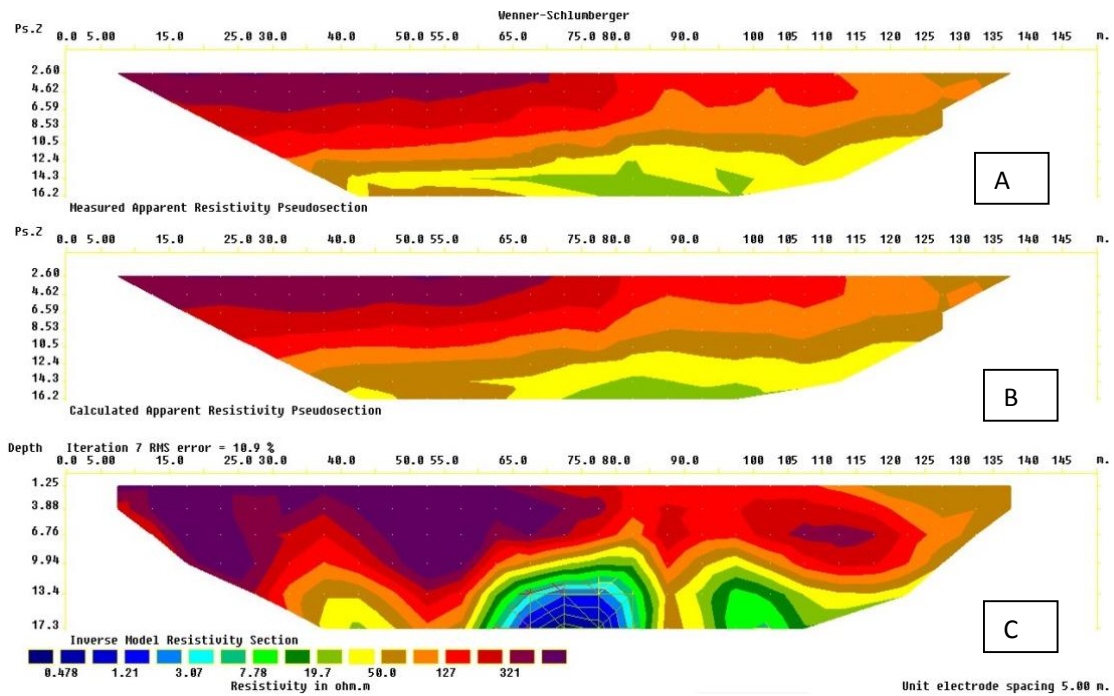
Fig. 5. Inverted 2D-resistivity section along traverse three
