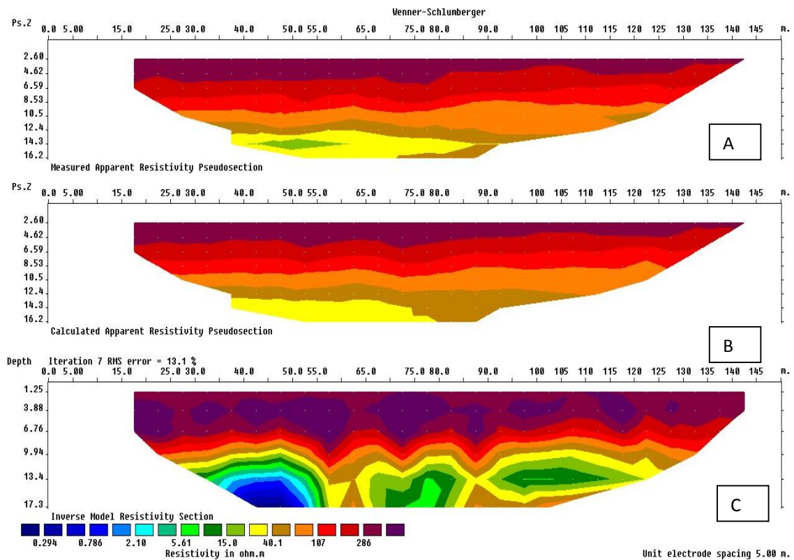
Fig. 6. Inverted 2D-resistivity section along traverse four
