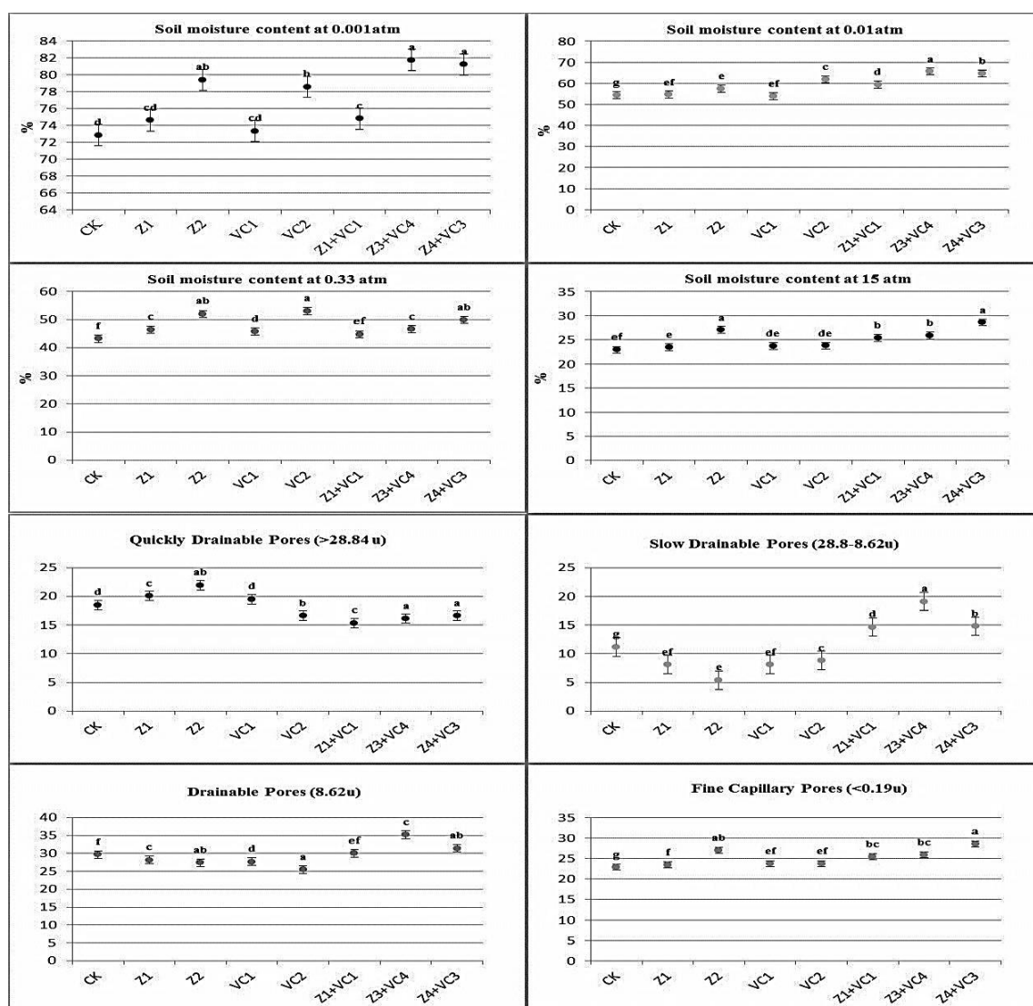
Fig. 2. Effect of different rates of zeolite, vermicompost and their combinations on soil moisture content and pores size distribution after both seasons. Different letters on the top of the bars indicate significant differences at P < 0.05
